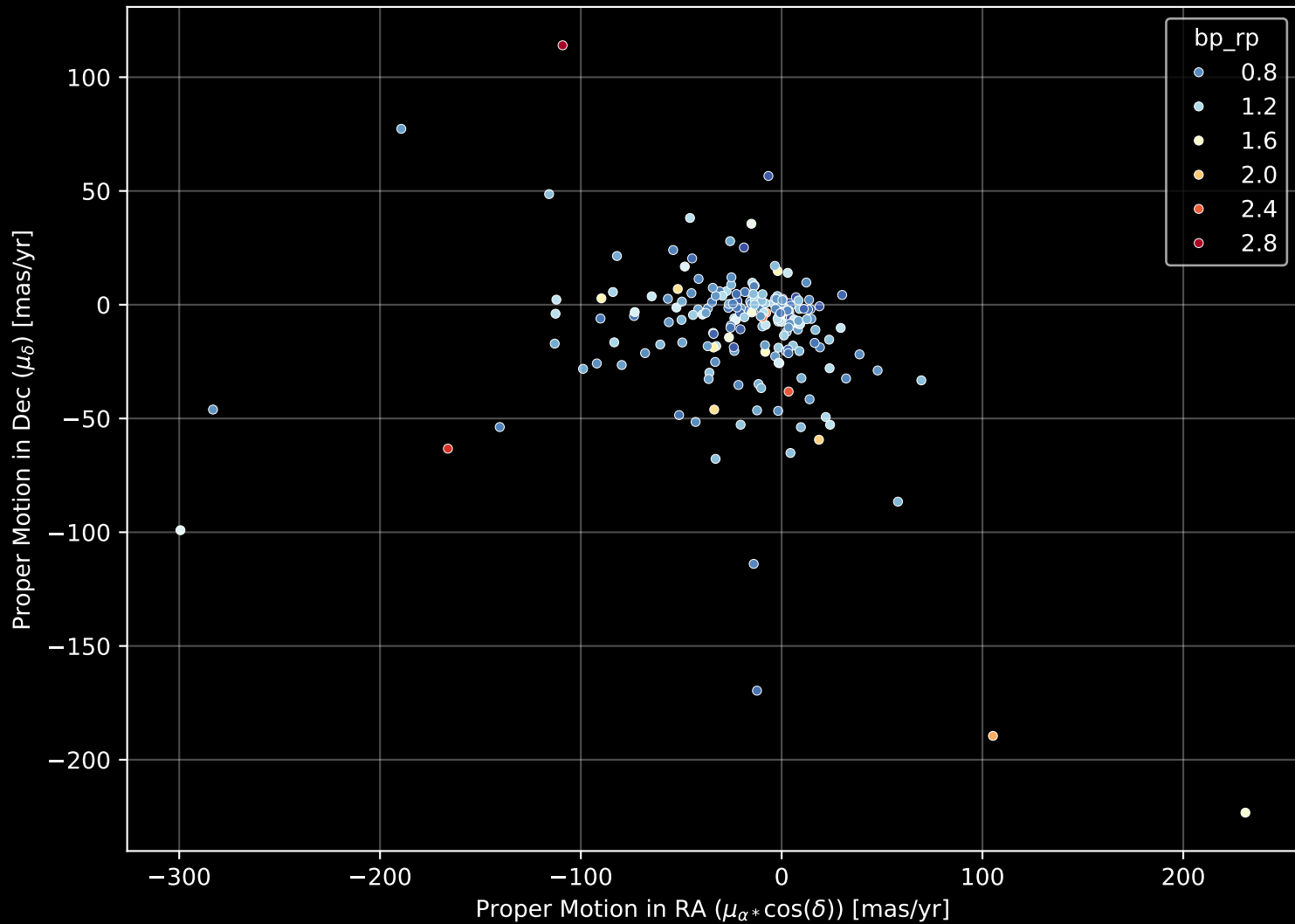
APOGEE DR17 Field: [141+72_MGA] Proper Motion Diagram (n= 201)
