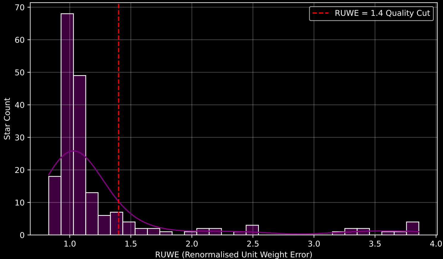
GAPOGEE DR17 Field [141+72_MGA] RUWE Distribution (n= 190)
