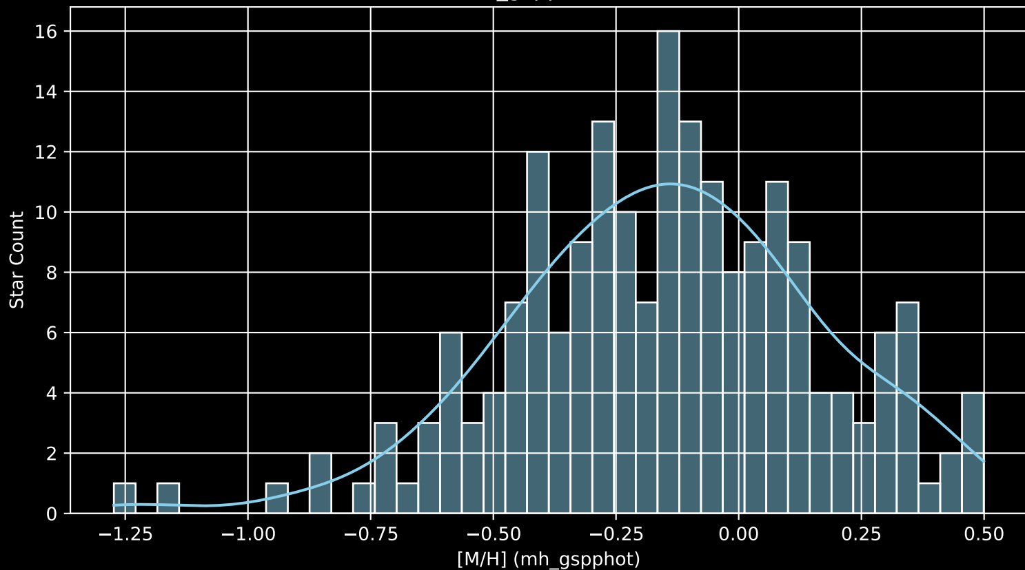
APOGEE DR17 Field: [141+72_MGA [M/H] (mh_gspphot) (n= 198)
