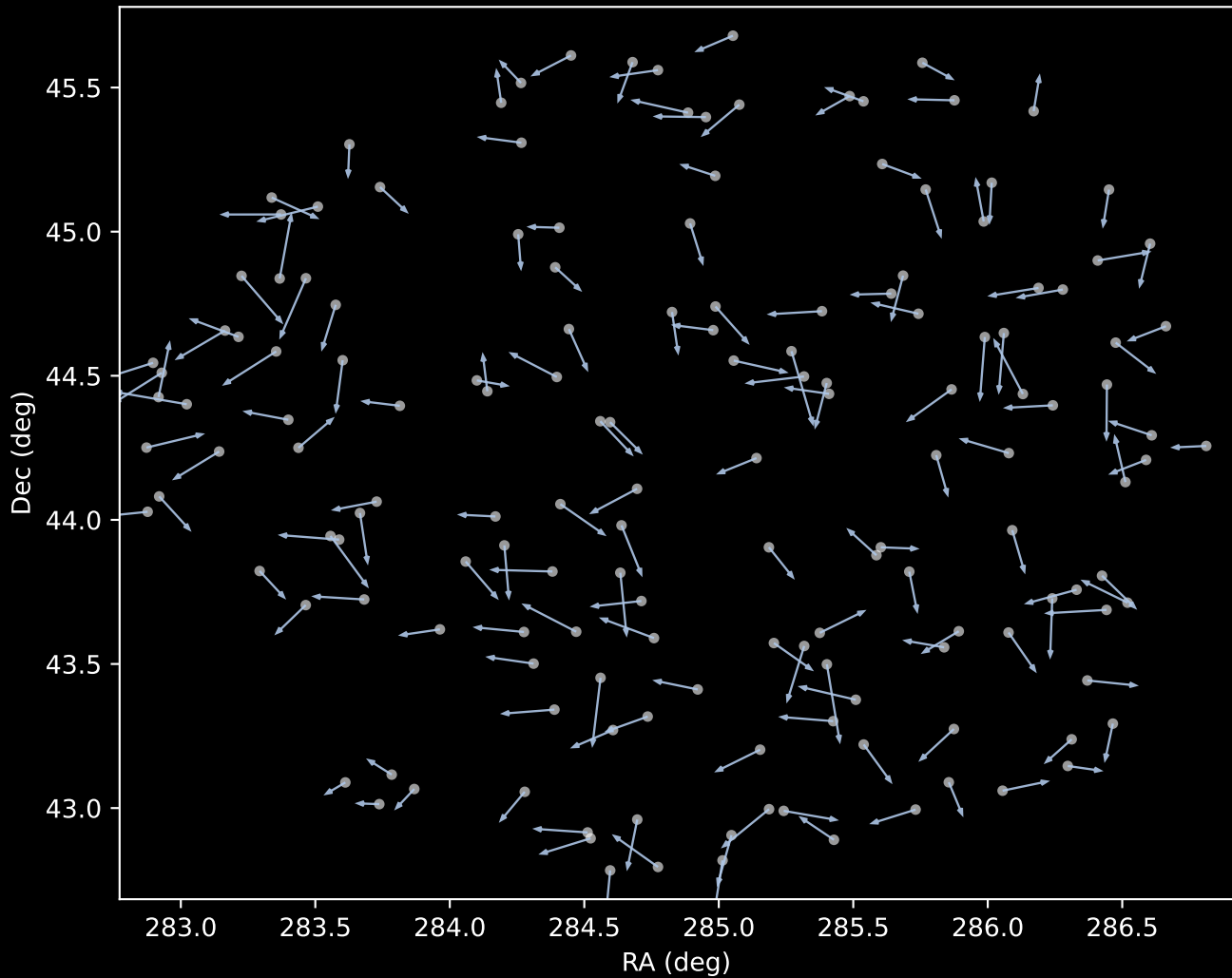
APOGEE DR17 Cluster 1 Proper Motion Vectors (n=156)
