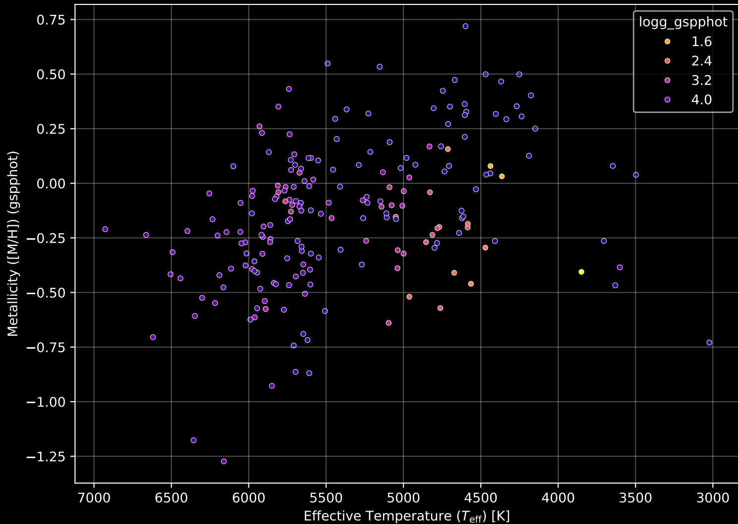
APOGEE DR17 Field: [141+72_MGA] Stellar Population Parameters (n= 201)
