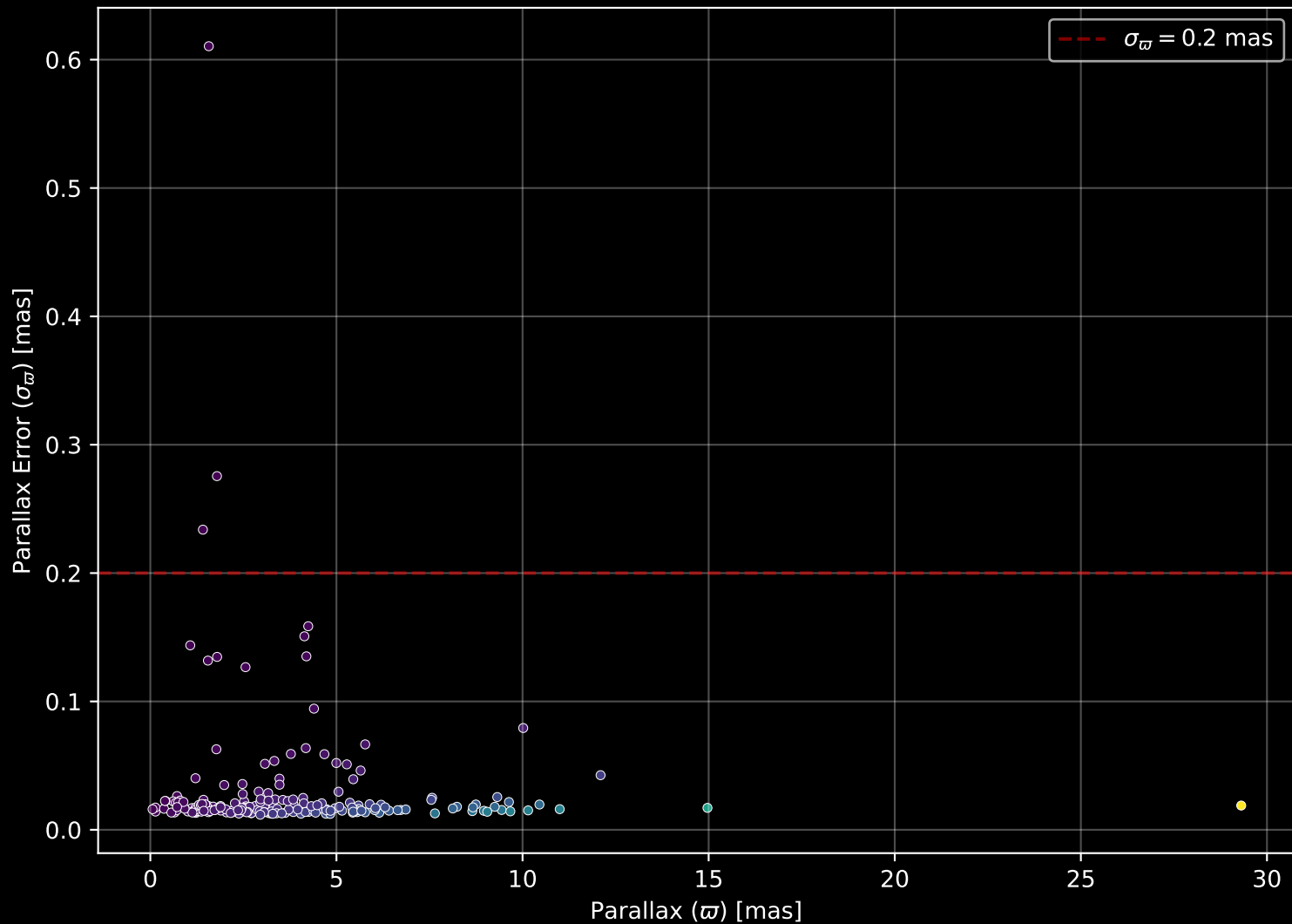
APOGEE DR17 Field: [141+72_MGA] Parallax Quality (n= 201)
