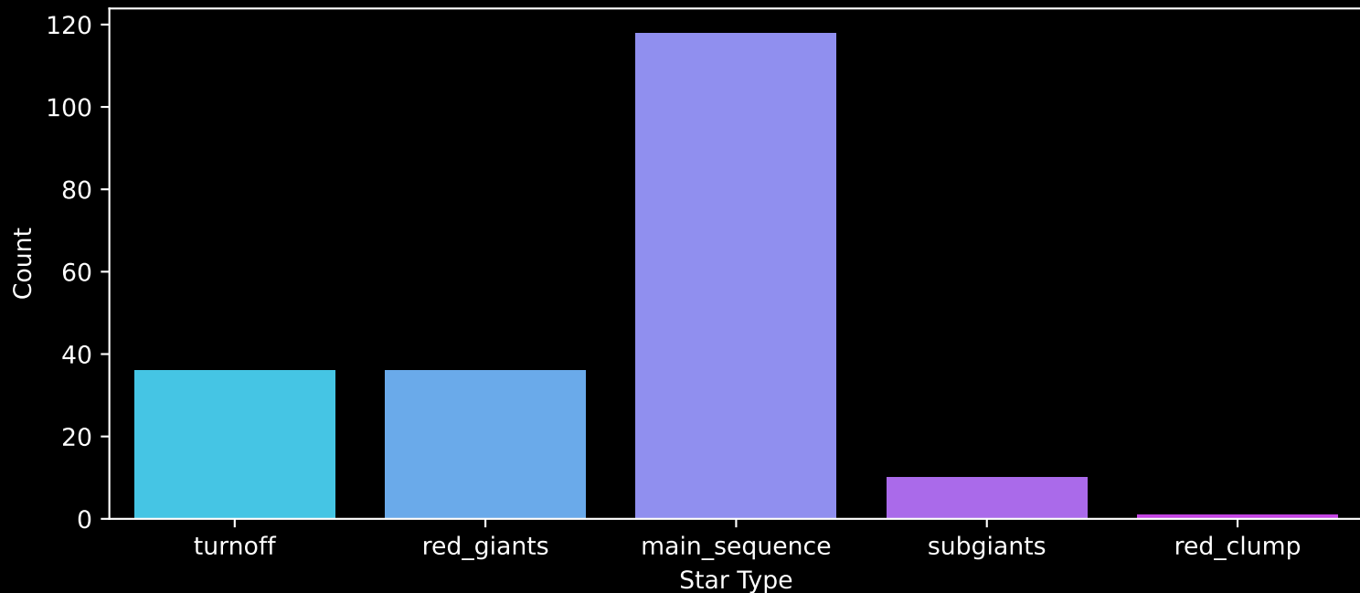
APOGEE DR17 Field: [141+72_MGA] Count plot of Star Type
